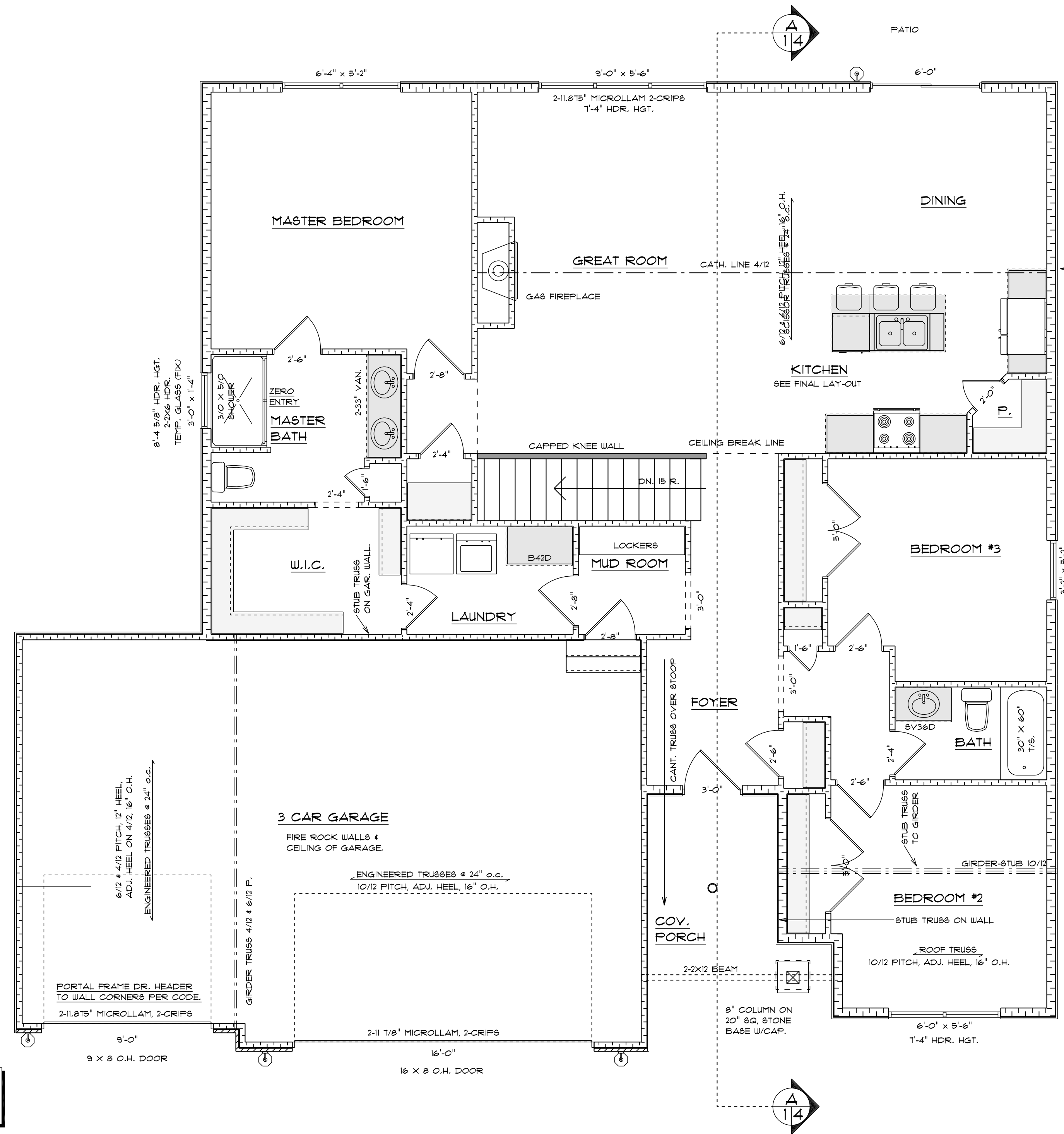
MAIN FLOOR SCALE: 1/4" = 1'-0"
