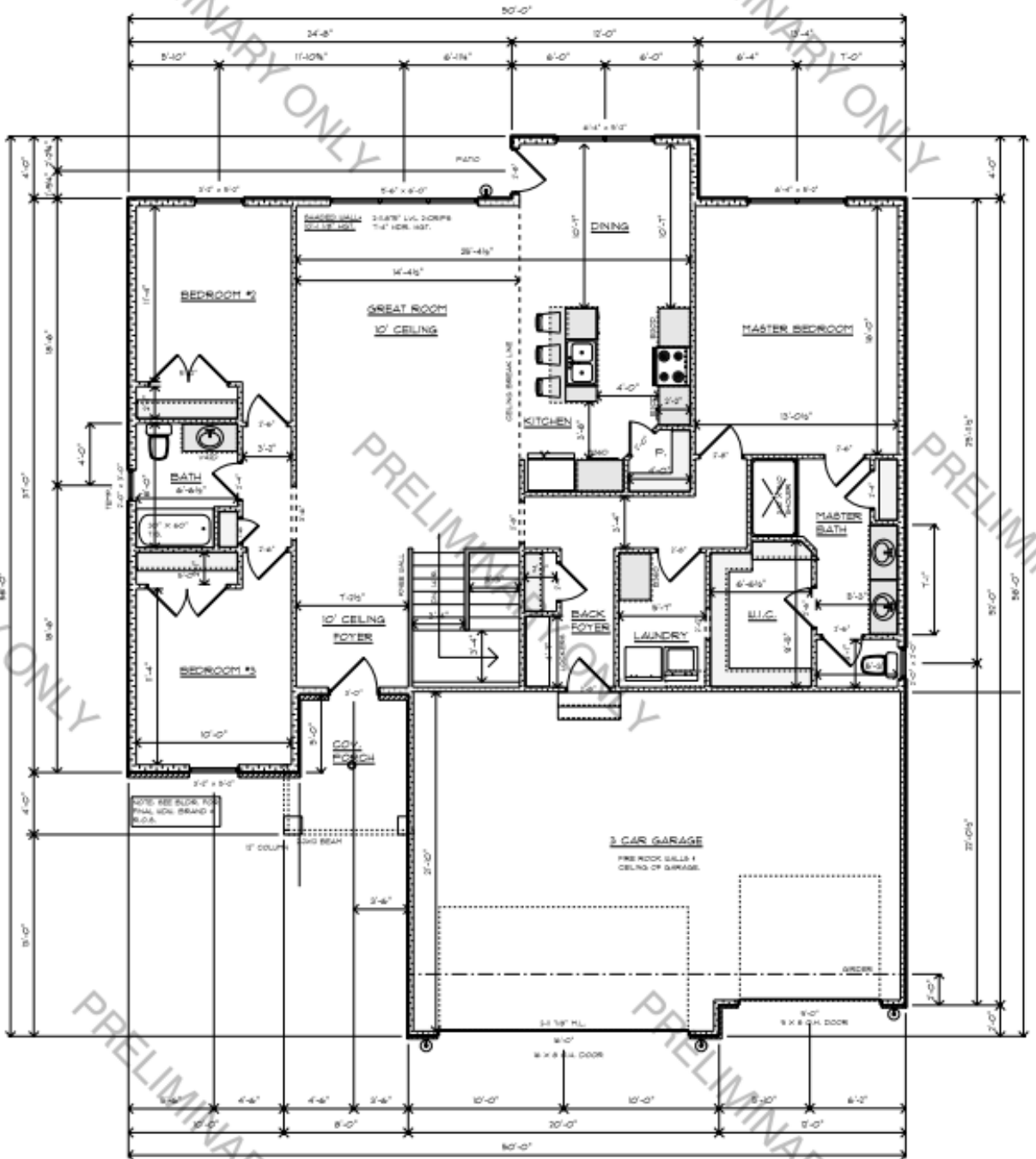
MAIN FLOOR SCALE: 1/4" = 1'-0"
